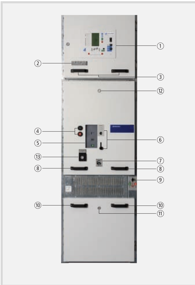
Circuit-breaker panel with operator interface
