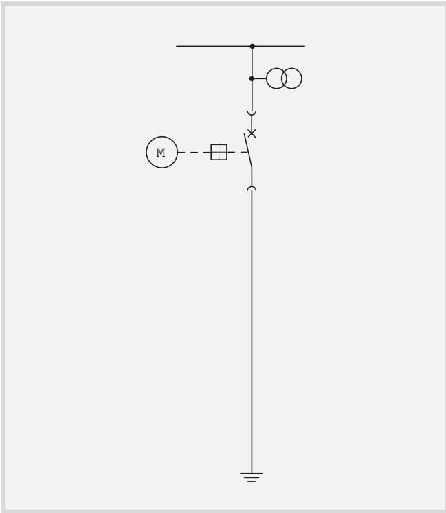
Configuration example for panel type ...-E Other equipment options → page 31.
