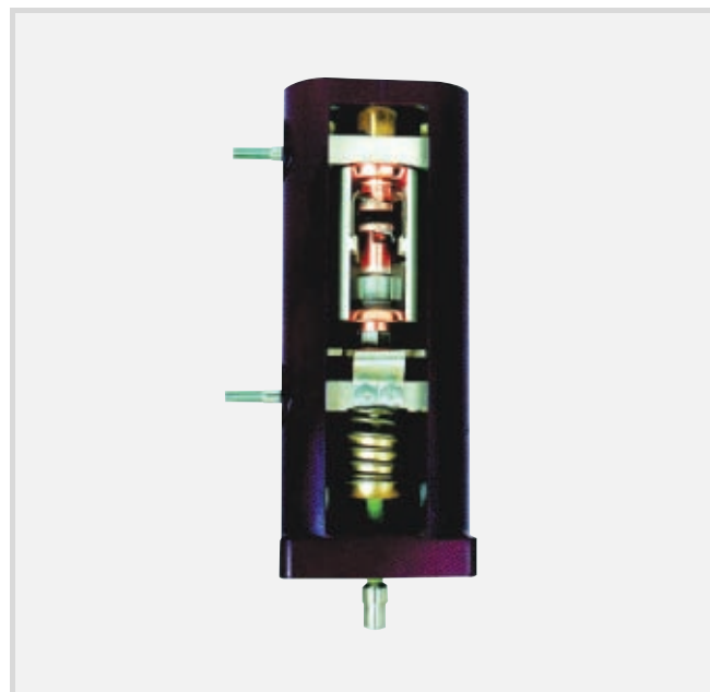
Switch pole with cast resin insulator and support
