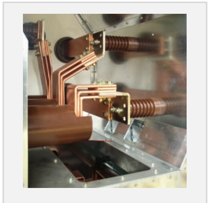
Busbar compartment with capacitive insulators
